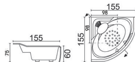
VIRGO ( 155 x 155 x 60cm )
