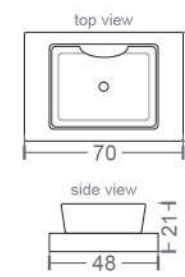
WM-8072A 70 x 48 x 21cm
