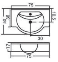
COSSY 75 75 x 50 x 17cm
