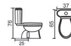
MINORA White Color 65 x 37 x 76 cm
