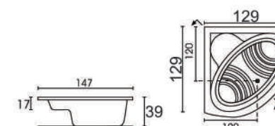
129 x 129 x 39cm ( L x W x H )
